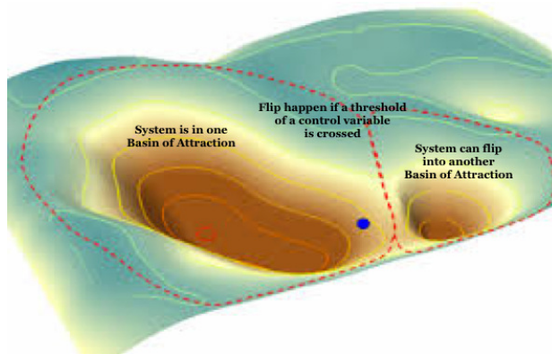
Fig. 1 Basin of attractions
